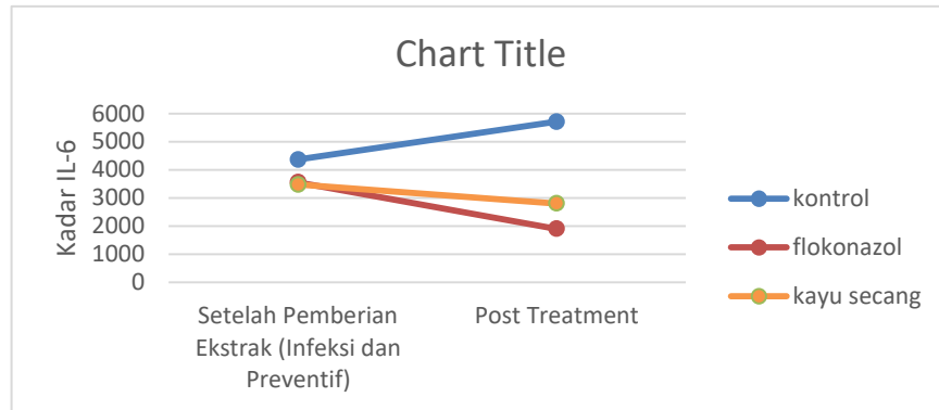
Graph 1 Profile of Interleukin 6 Levels during the study
