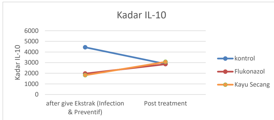
Graph 2 Profile of Interleukin 10 Levels during the study
